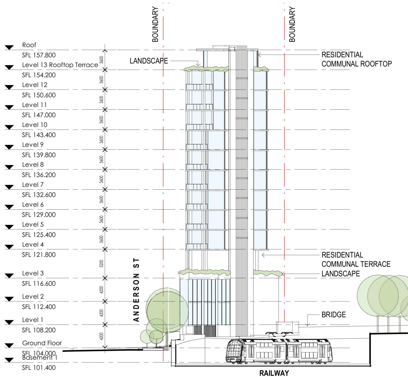
1 NORTH ELEVATION 1 : 400
